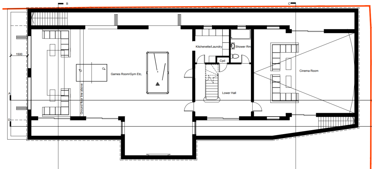
Proposed Basement
