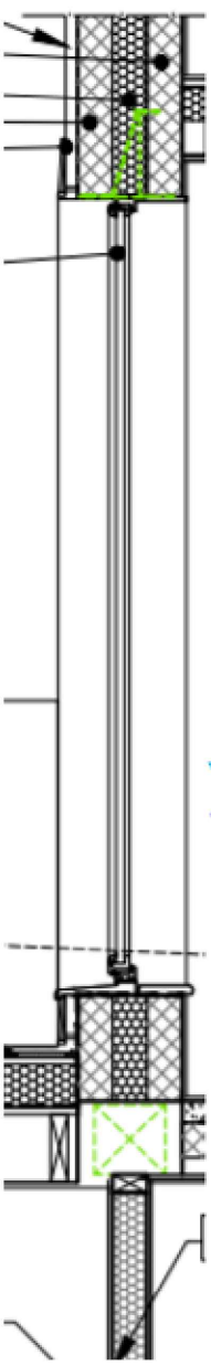
EXTERNAL WALL STRIP SECTION
