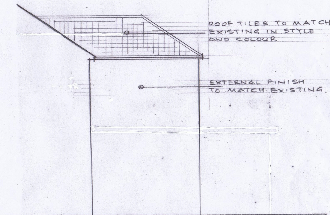
SIDE ELEVATION (PROPOSED) 1:50
