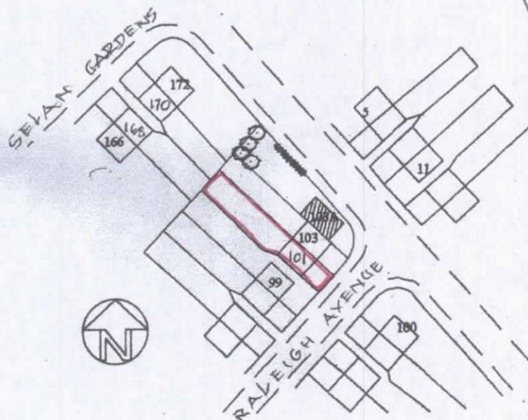
LOCATION PLAN 1/1250
