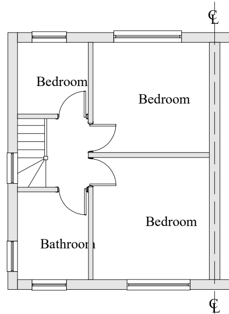
EXISTING FF PLAN
