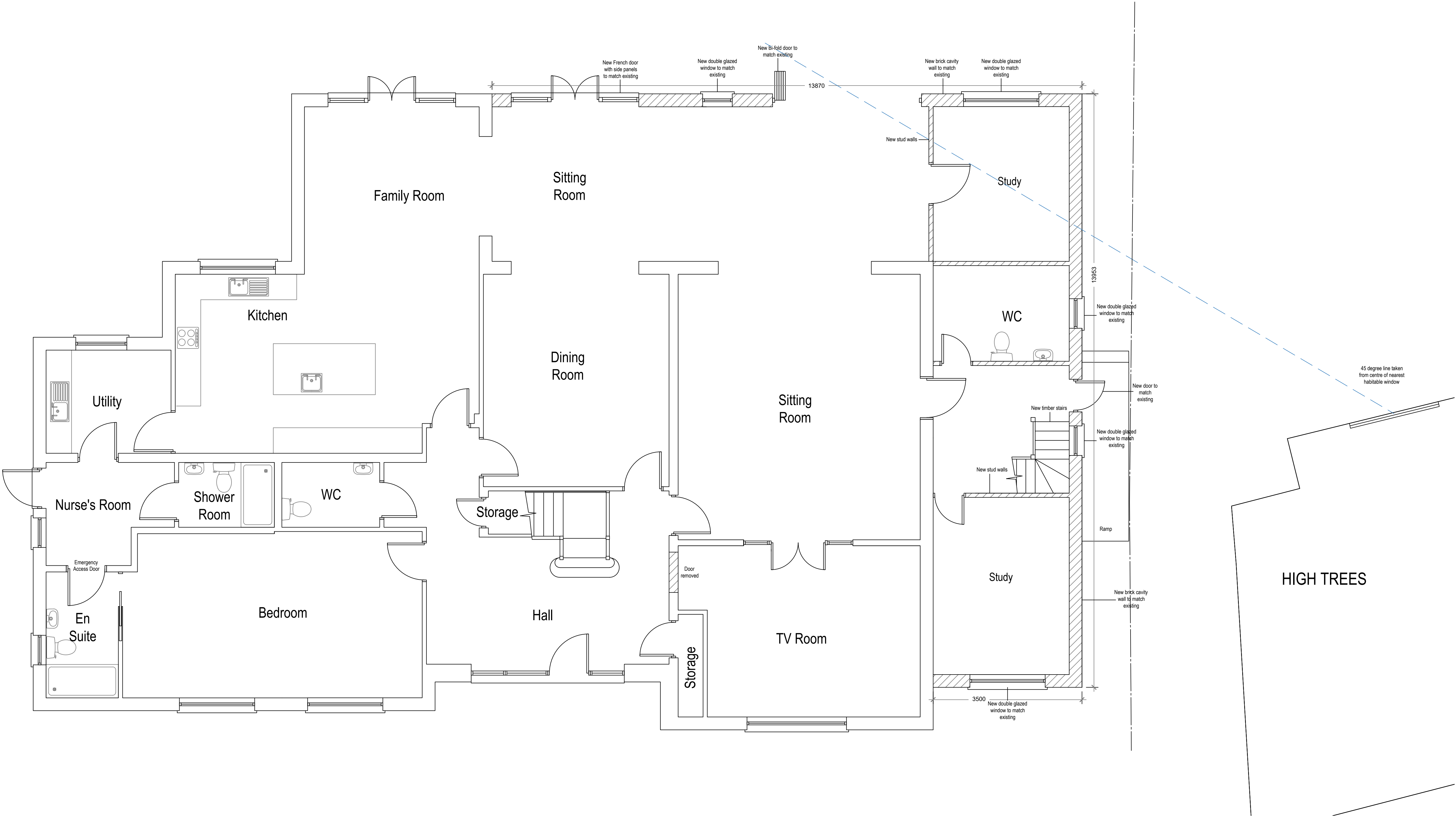
Proposed Ground Floor Plan Scale 1:50
