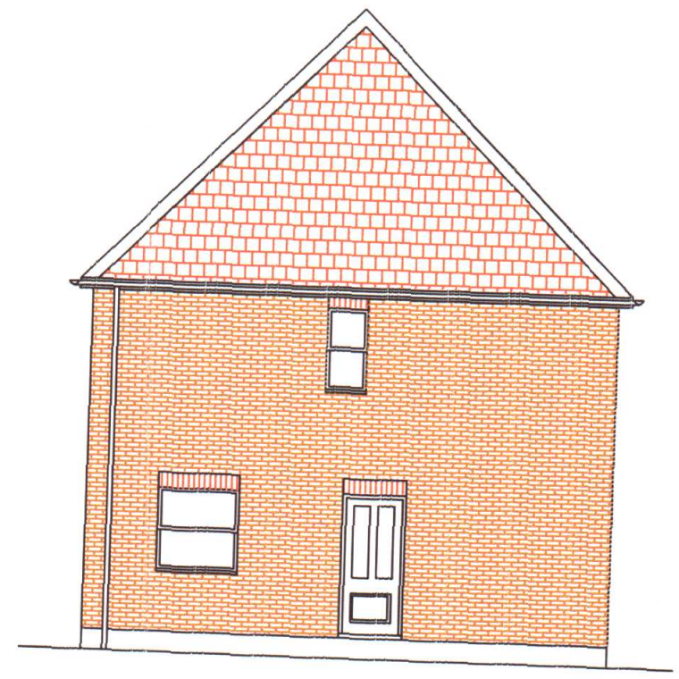
SIDE ELEVATION (WEST)
