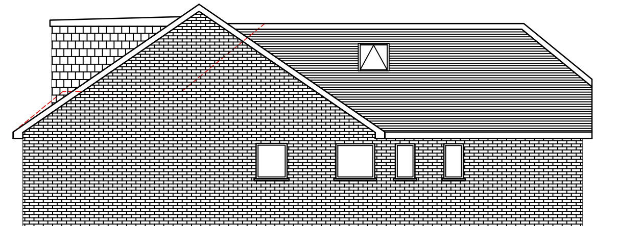
SIDE ELEVATION PROPOSED (AS VIEWED FROM NO:30)
