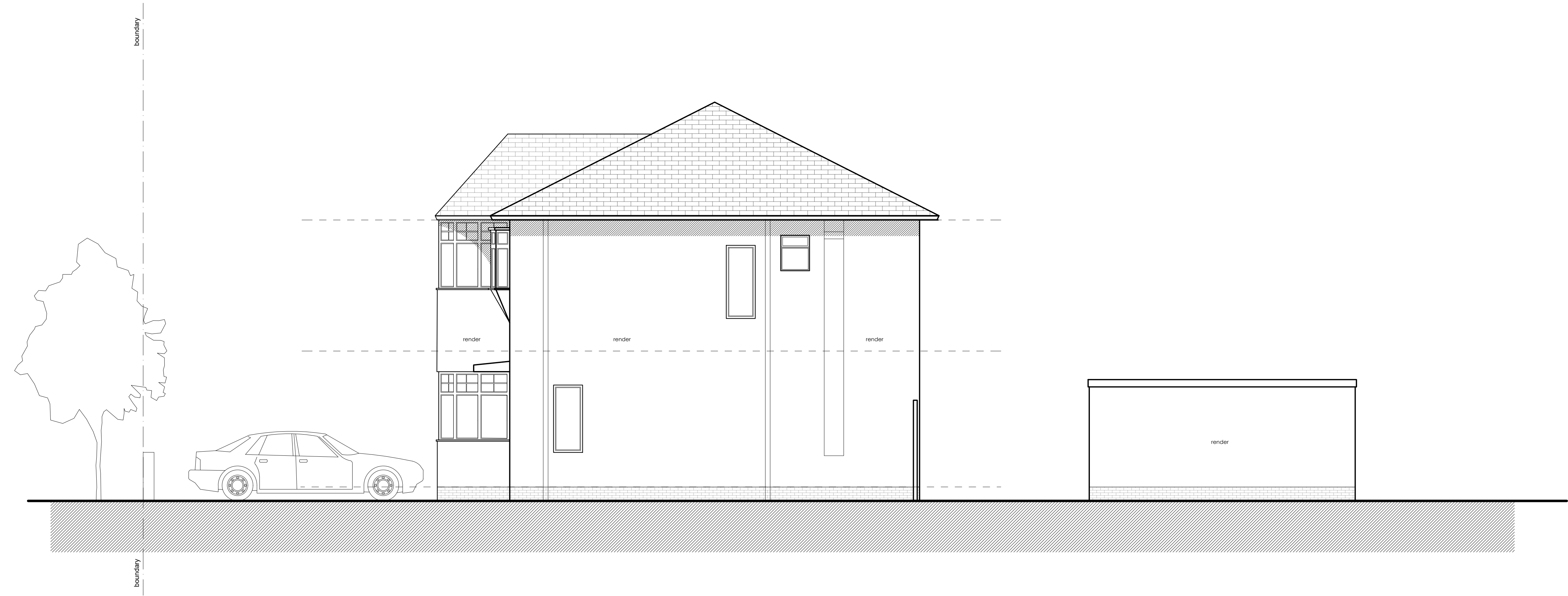
EXISTING SIDE ELEVATION A 1:50 Scale
