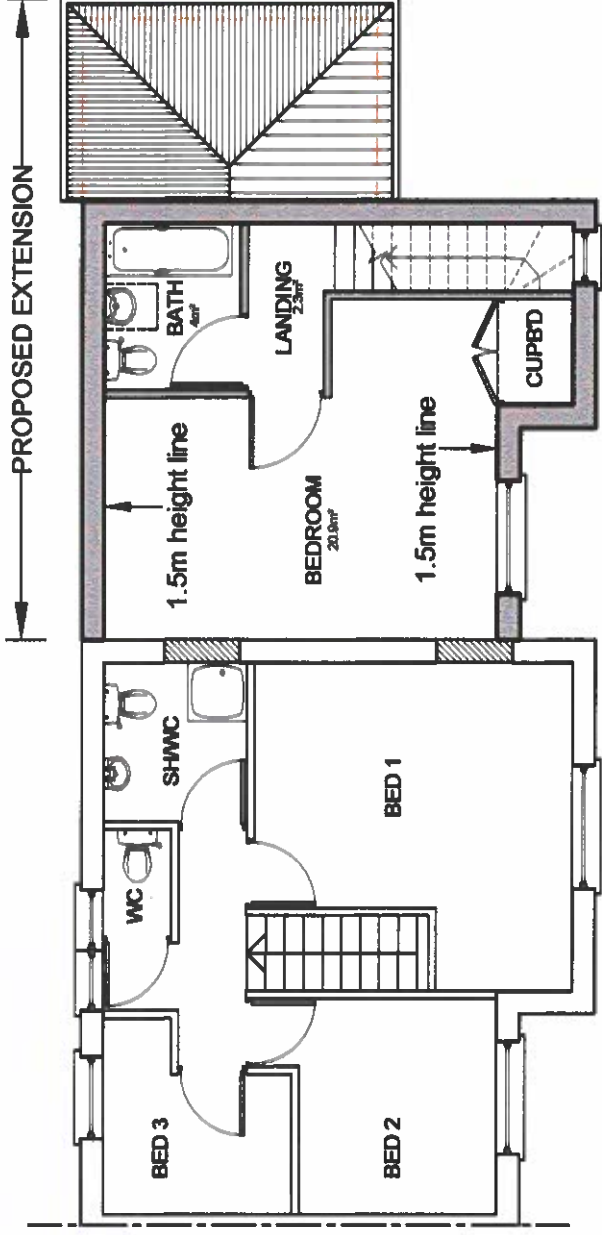
FIRST FLOOR PLAN GIA = 31m 2
