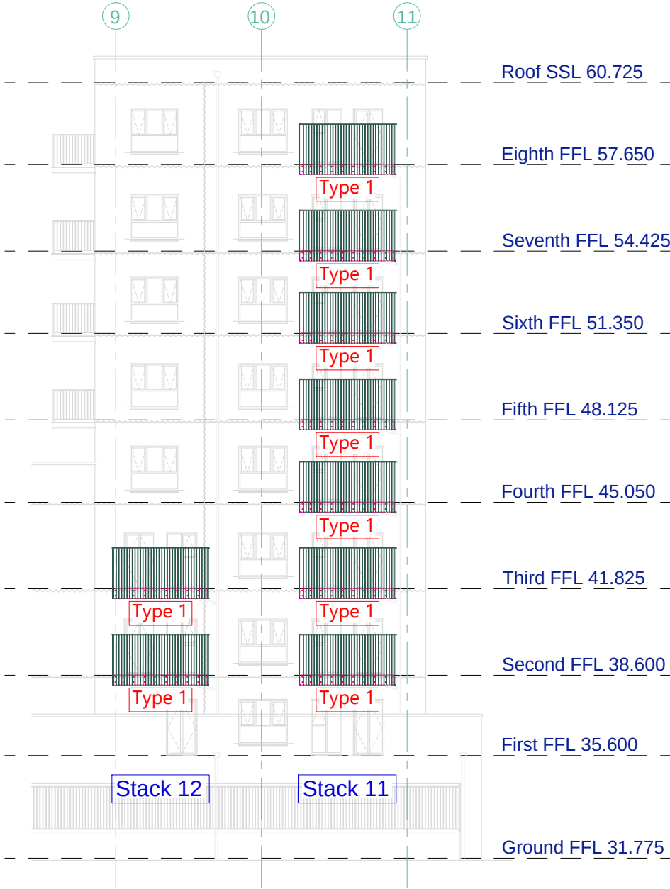
SOUTH EAST ELEVATION - ELEVATION 7
