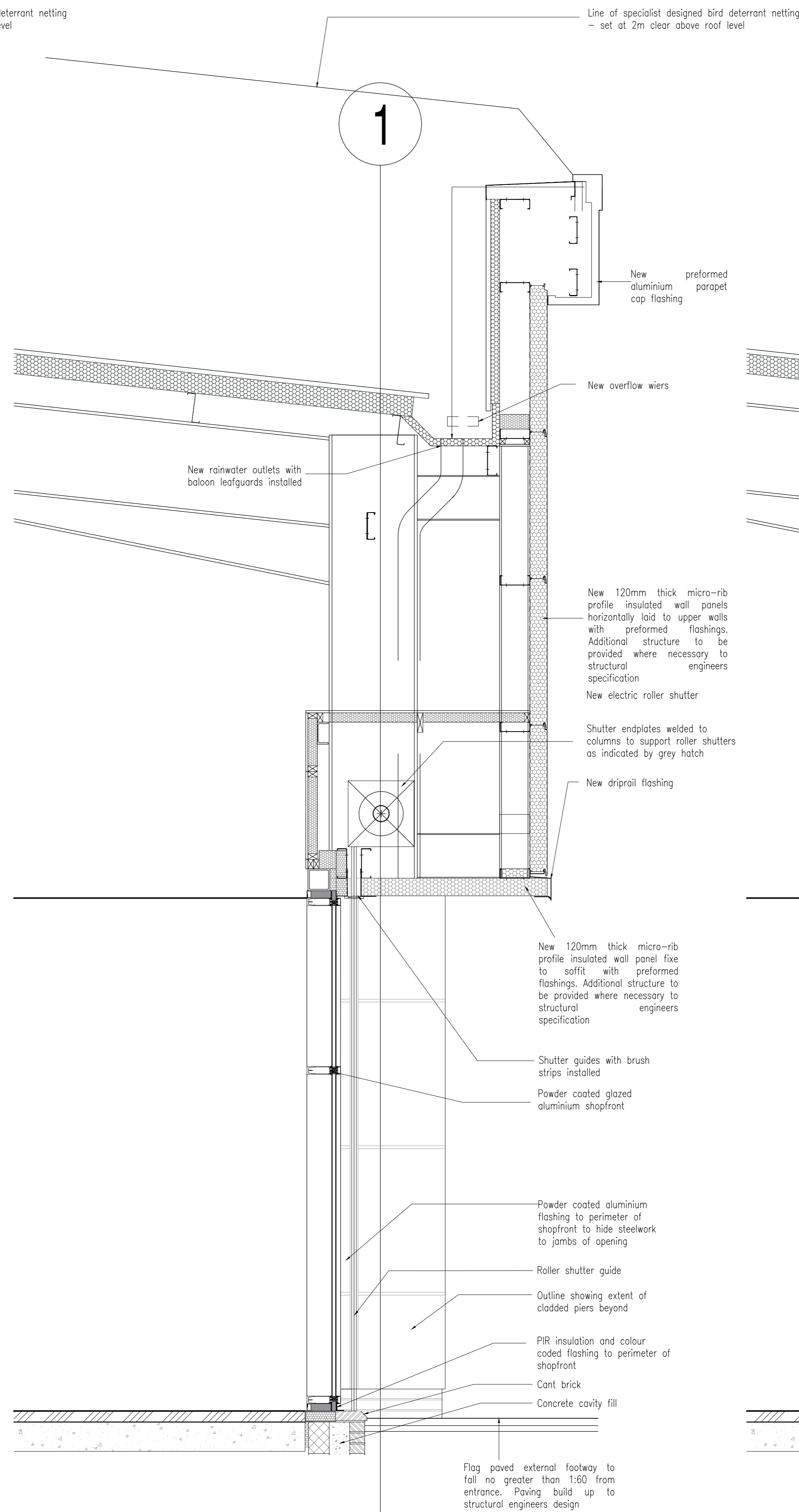
SECTION 2-2 1:20
