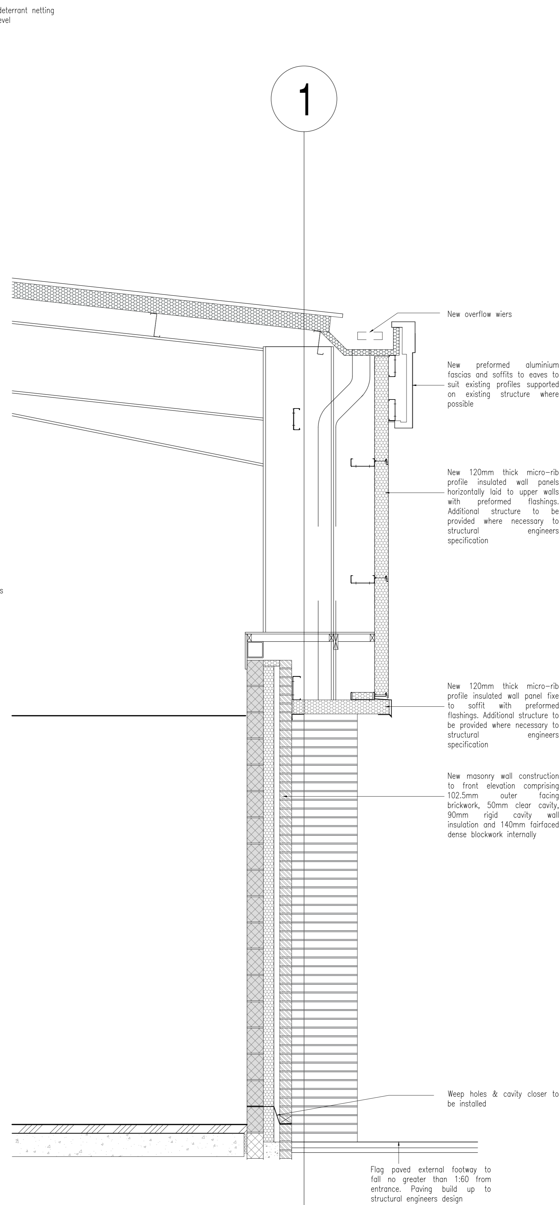
SECTION 3-3 1:20
