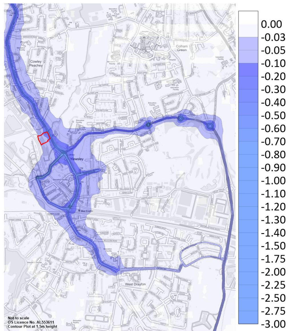
Figure 6-1. Annual Average Long-Term Nitrogen Dioxide (NO 2 ) Contribution from Proposed Development (µg/m 3 )
