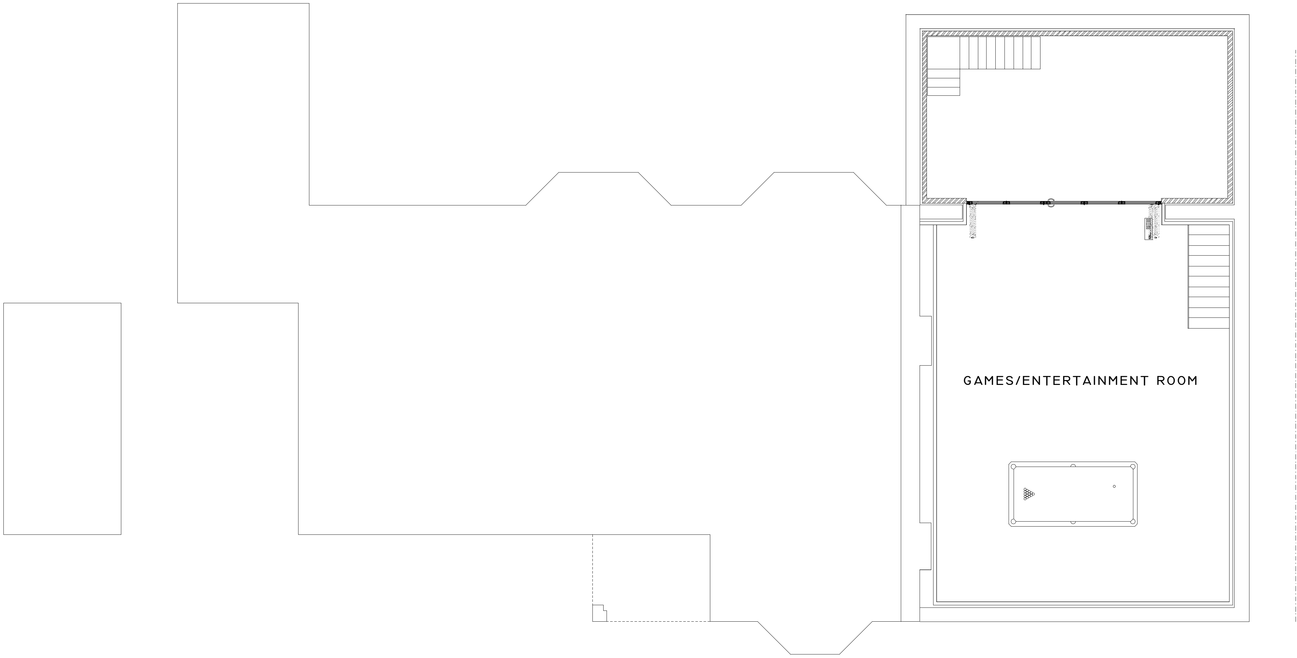
PROPOSED BASEMENT PLAN
