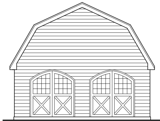
1:100 PROPOSED NORTH ELEVATION
