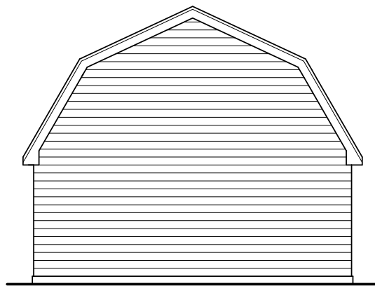
1:100 PROPOSED SOUTH ELEVATION
