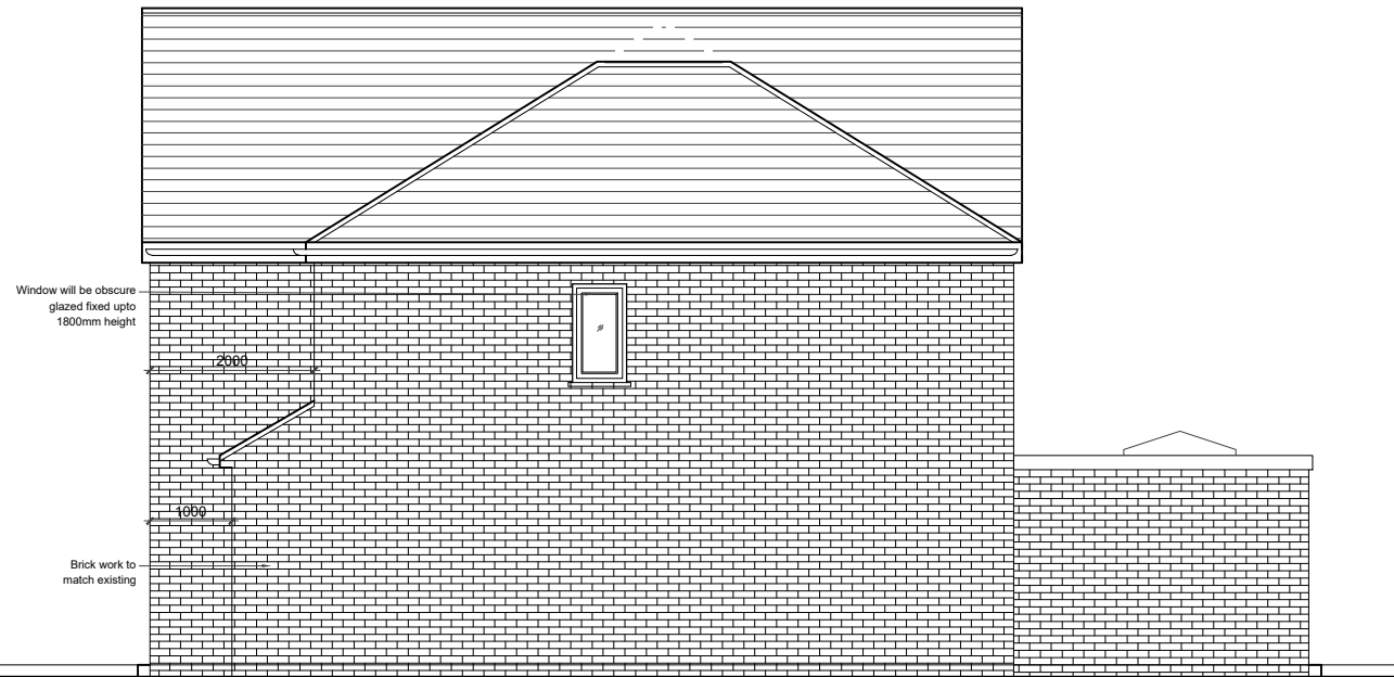
03 - SIDE ELEVATION
