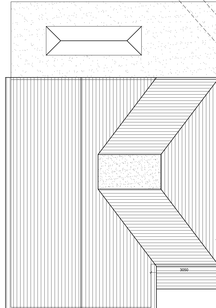
03 - ROOF PLAN
