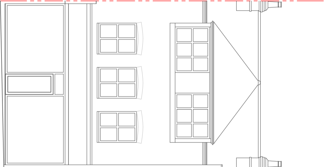
EXISTING & PROPOSED FRONT ELEVATION
