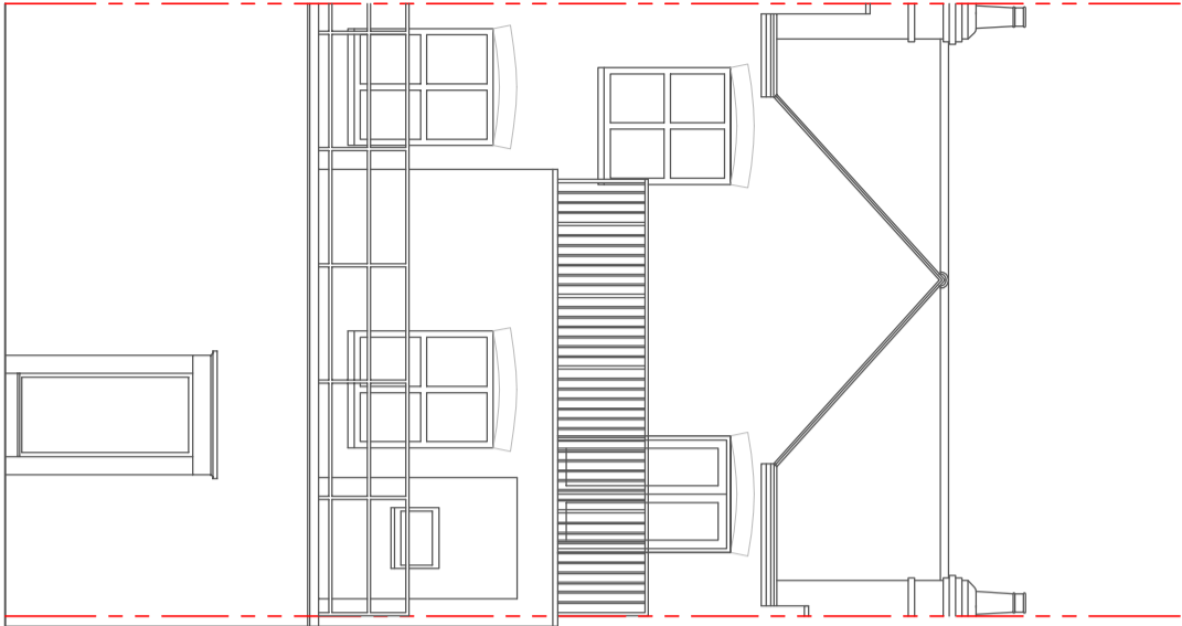
EXISTING & PROPOSED REAR ELEVATION
