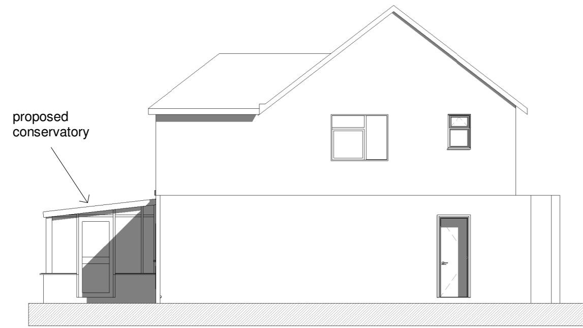
South elevation (proposed) 1 : 100
