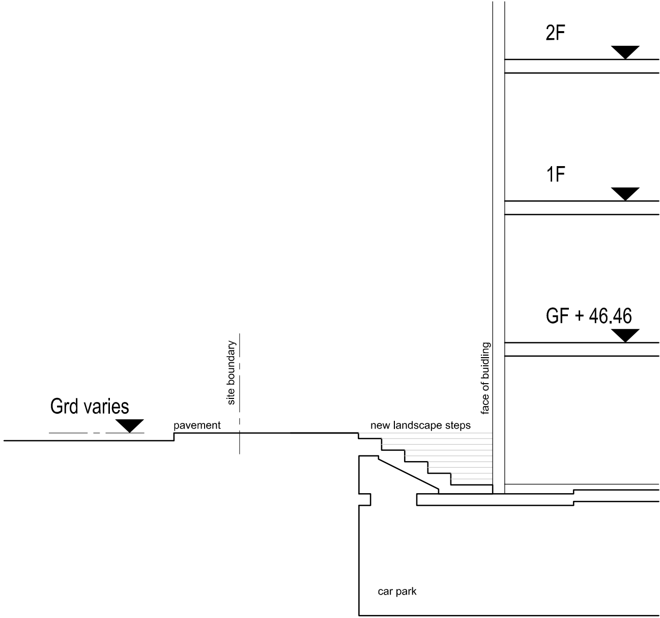
SECTION A
