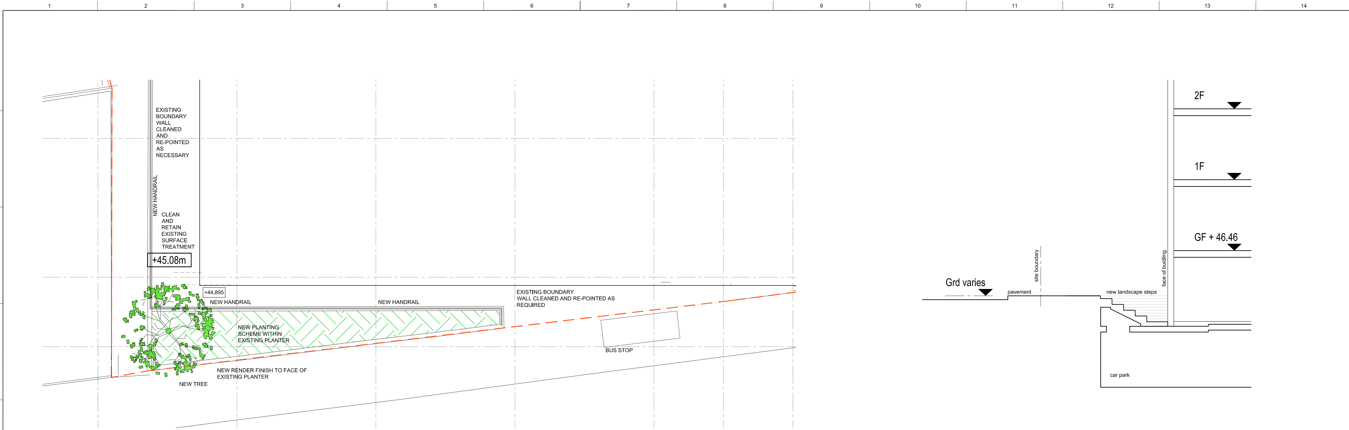
A. PART PLAN ALONG BELMONT ROAD FRONTAGE scale 1:100
