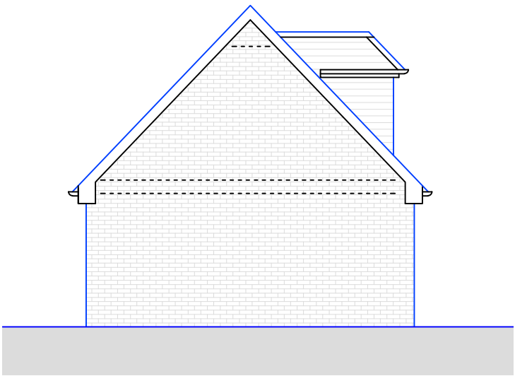
○ Side Elevation 2 1 : 1 0 0
