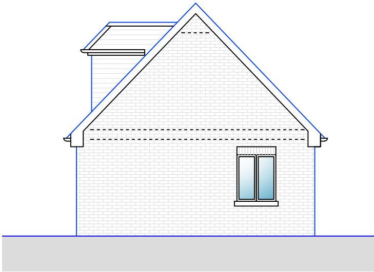
○ Side Elevation 1 1 : 1 0 0
