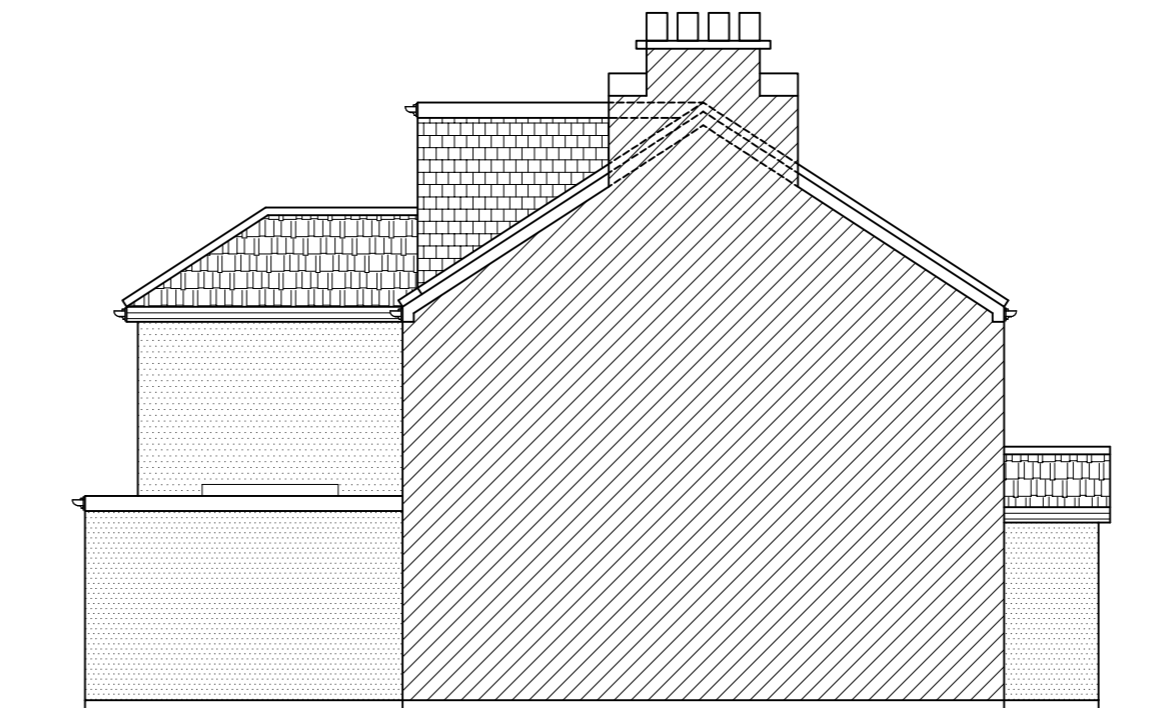
EXISTING SIDE ELEVATION -02
