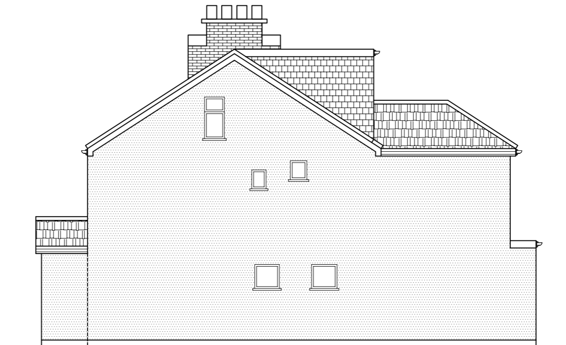
EXISTING SIDE ELEVATION -01
