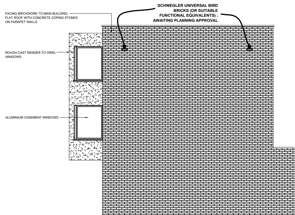
SIDE ELEVATION PROPOSED (AS VIEWED FROM NO: 1-6 RUSSET CLOSE)
