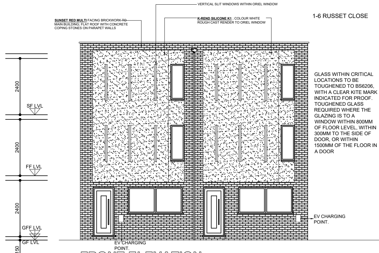
FRONT ELEVATION PROPOSED
