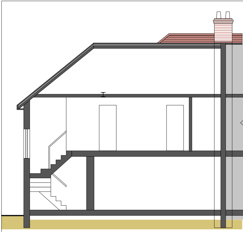
SECTION C-C - AS EXISTING
