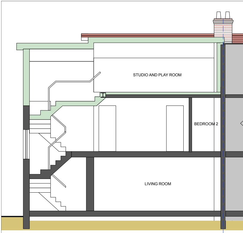
SECTION C-C - AS PROPOSED
