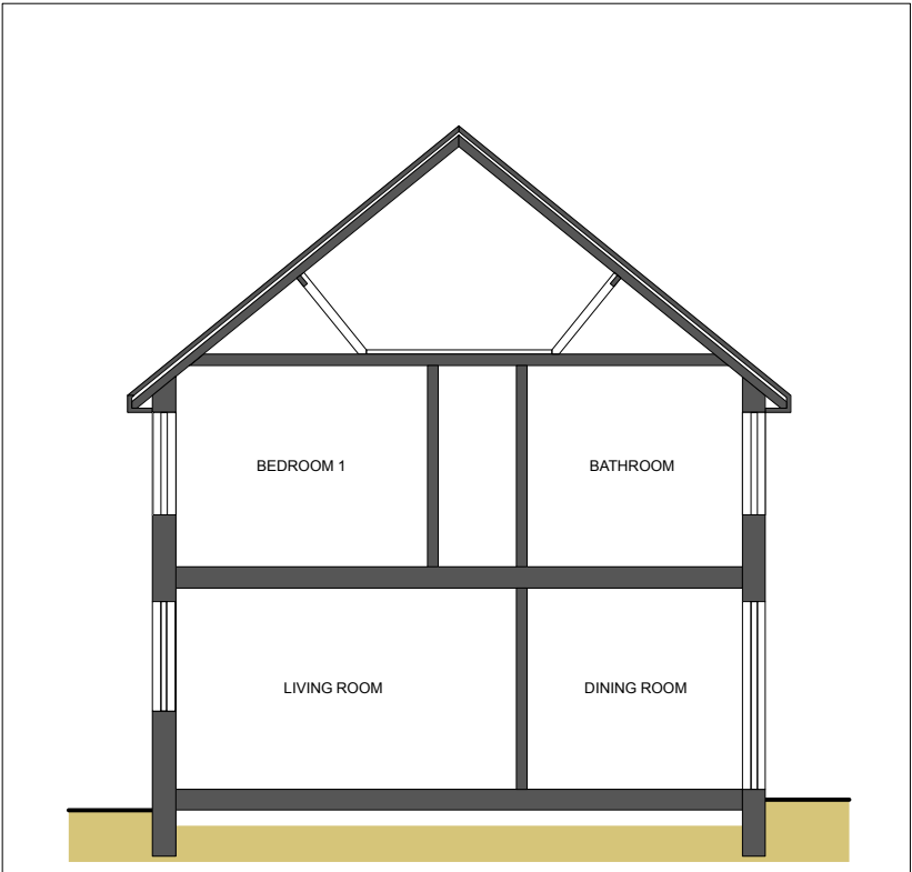
SECTION B-B - AS EXISTING
