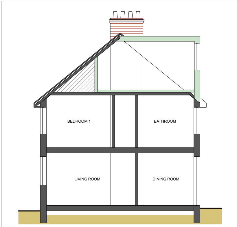
SECTION B-B - AS PROPOSED
