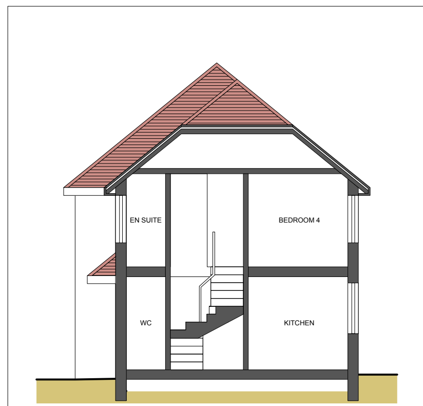
SECTION A-A - AS EXISTING
