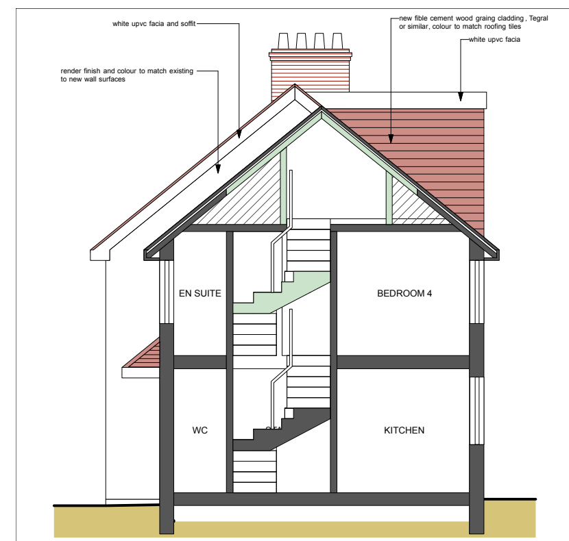
SECTION A-A - AS PROPOSED
