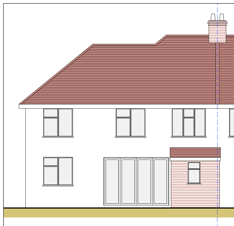
BACK ELEVATION - AS EXISTING
