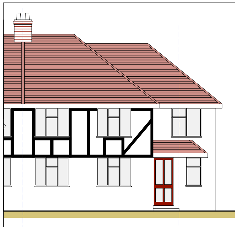
FRONT ELEVATION - AS EXISTING
