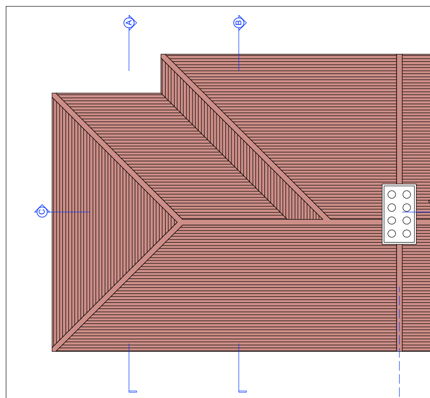
ROOF PLAN - AS EXISTING
