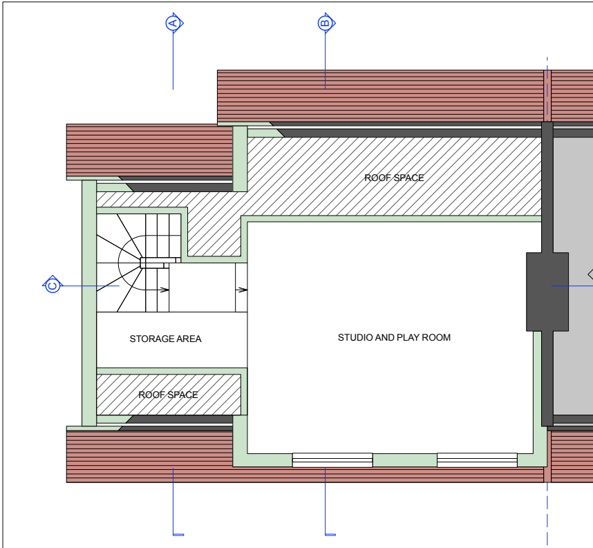
SECOND FLOOR PLAN - AS PROPOSED
