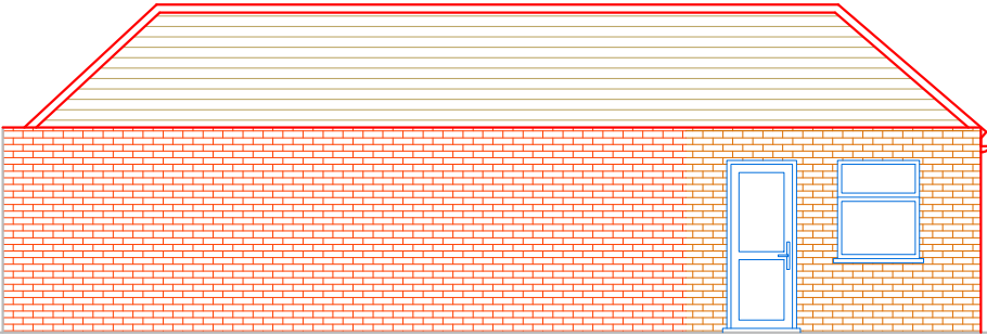
PROPOSED SIDE ELEVATION-2
