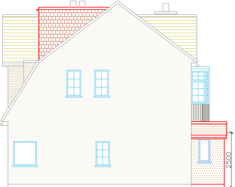
PROPOSED SIDE ELEVATION-2
