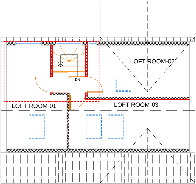
PROPOSED LOFT PLAN
