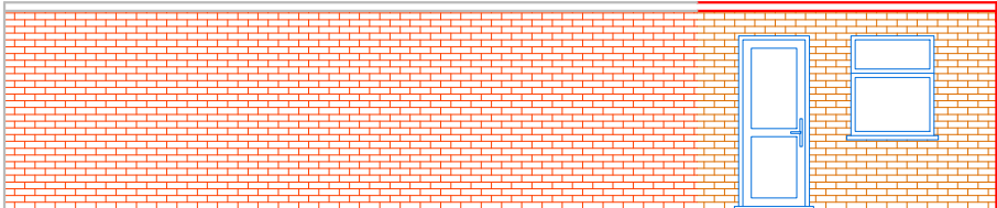
PROPOSED SIDE ELEVATION-2
