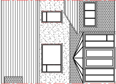
Existing Rear Elevation Scale 1:100
