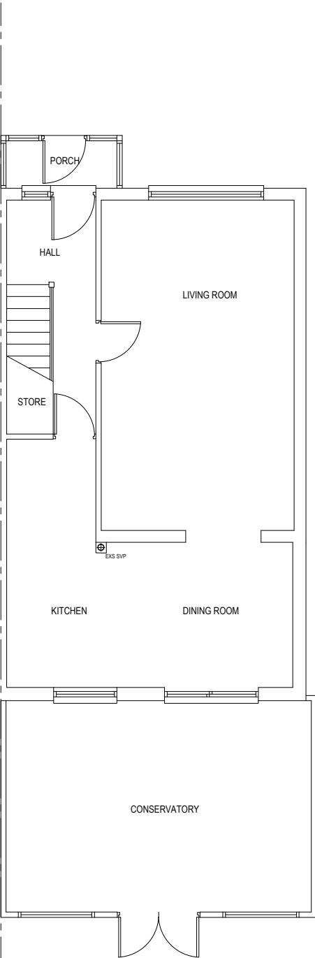
PROPOSED GROUND FLOOR
