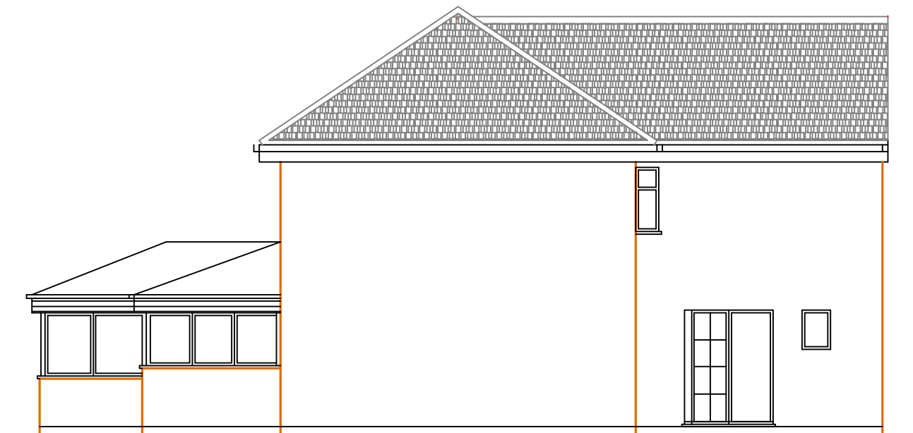
Existing east side elevation
