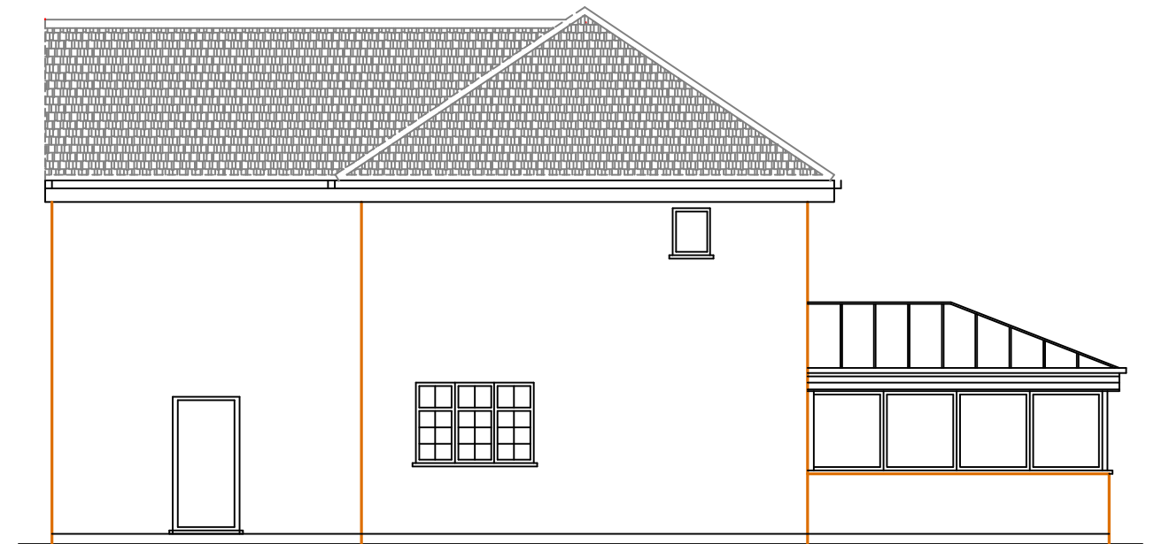
Existing west side elevation
