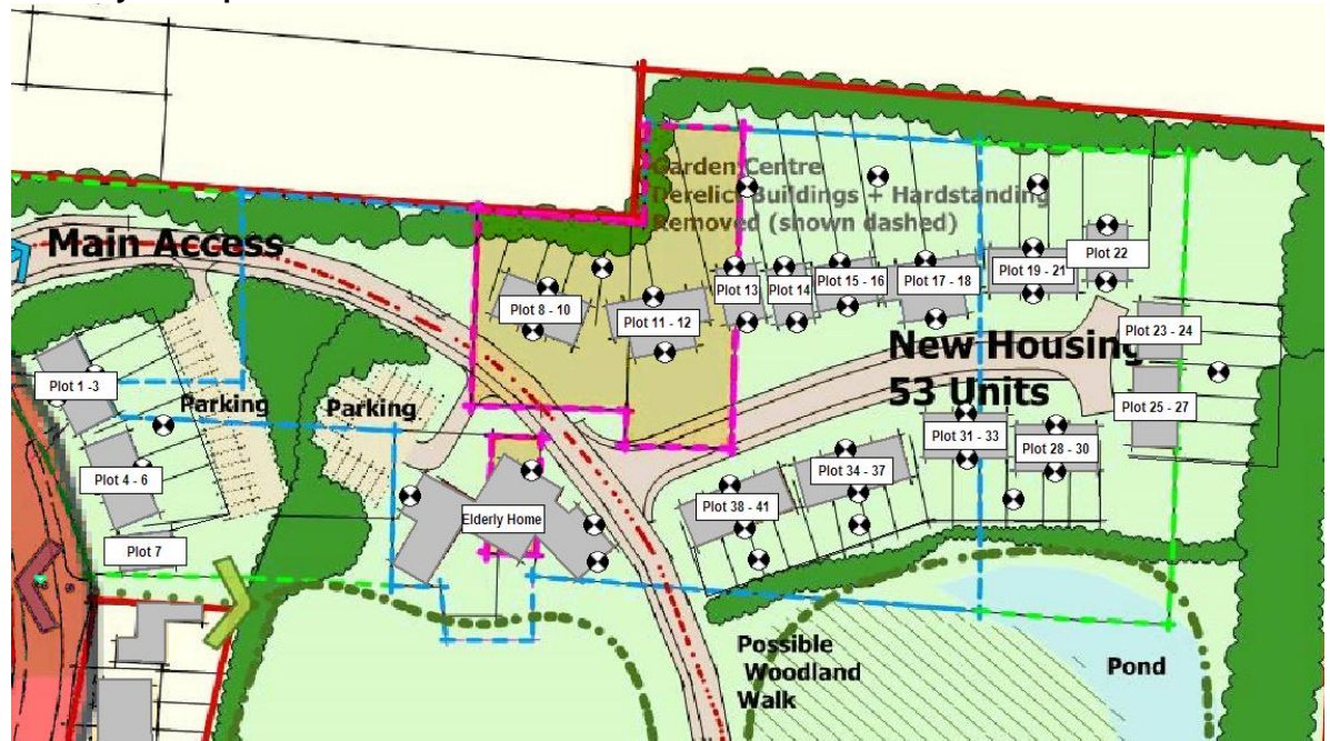
Figure 7: Layout of plot numbers for calculations
