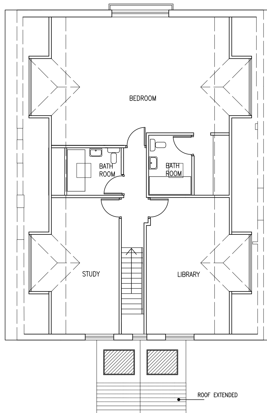
LOFT FLOOR PLAN PROPOSED
