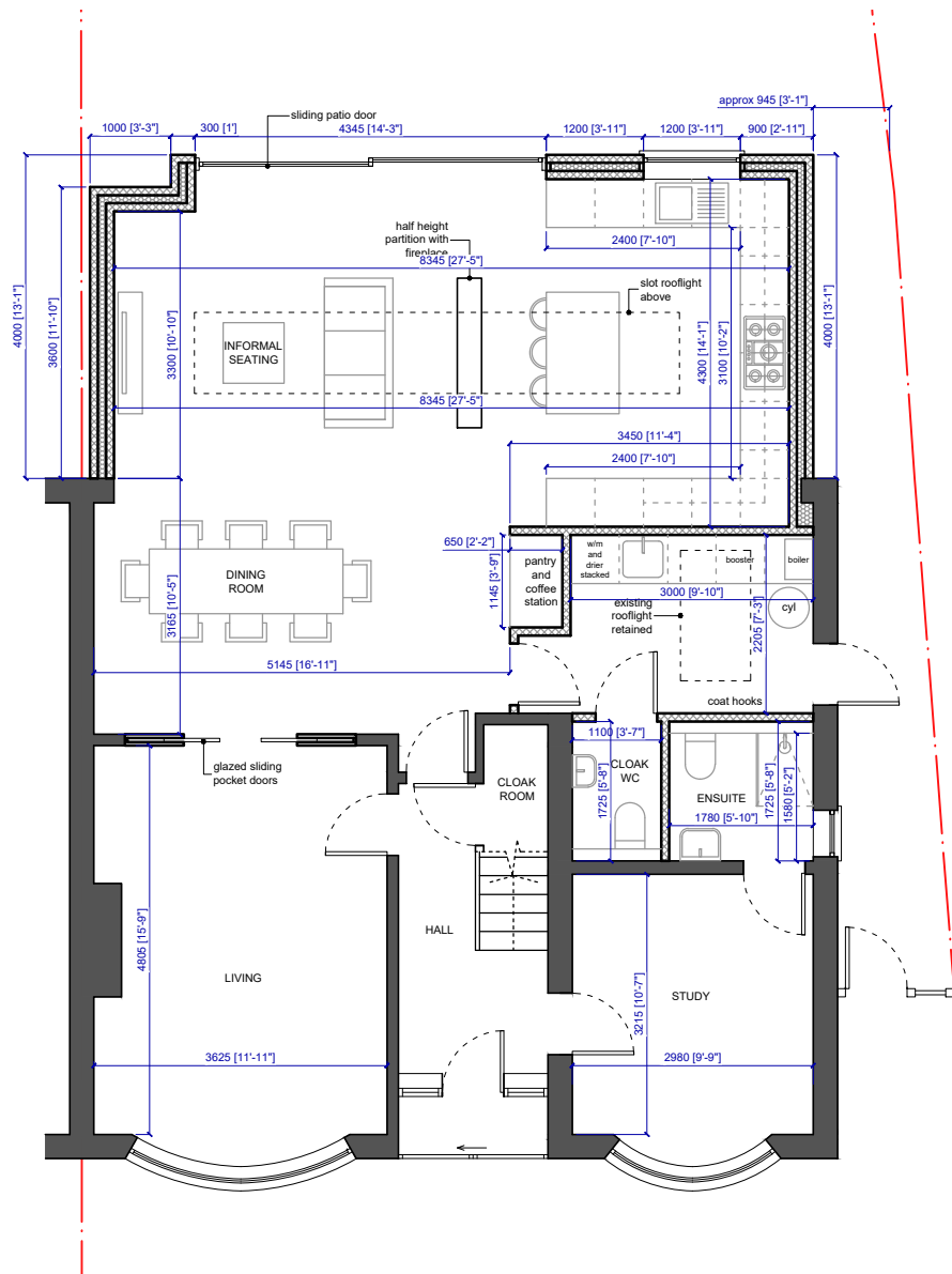
1 PROPOSED GROUND FLOOR
