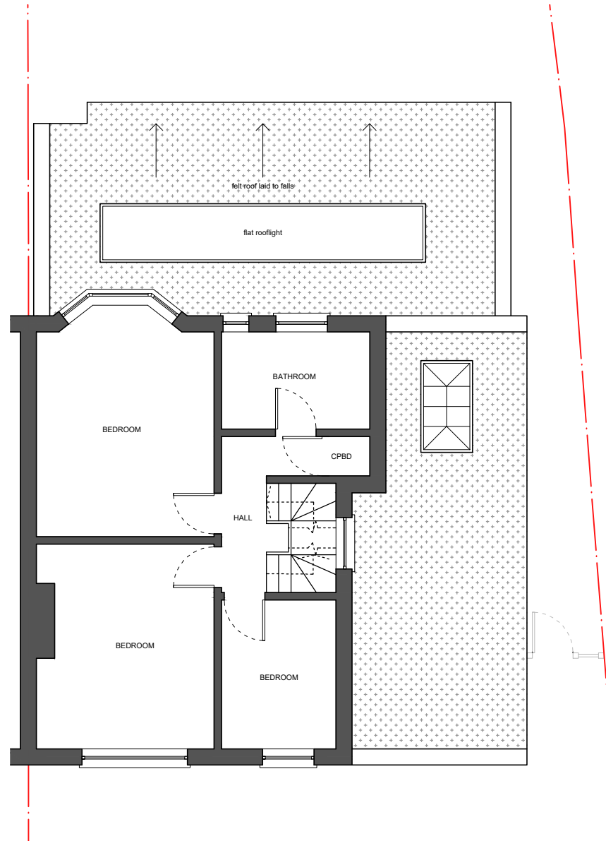
2 PROPOSED FIRST FLOOR
