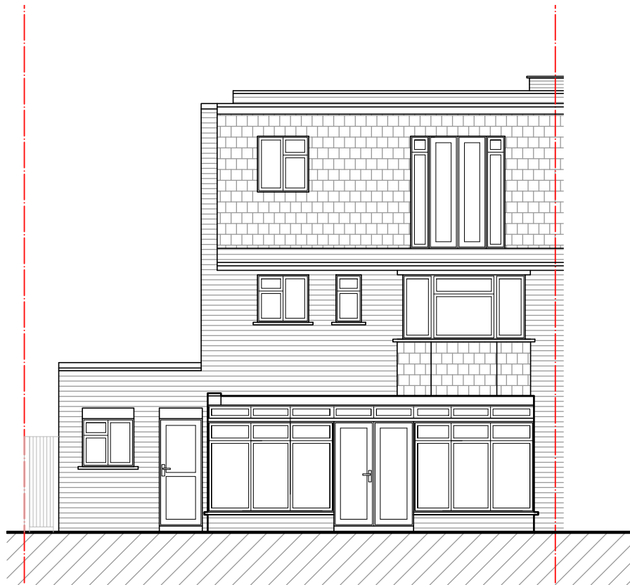
3 EXISTING REAR ELEVATION
