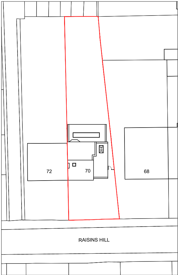
2 PROPOSED SITE PLAN
