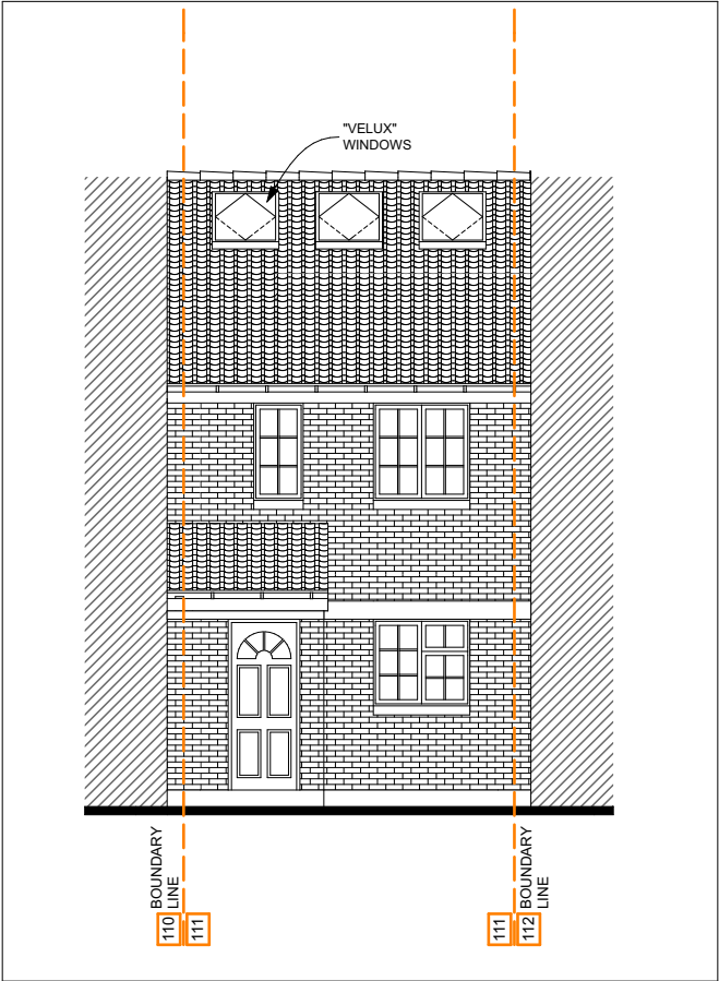
FRONT ELEVATION PROPOSED 1:100
