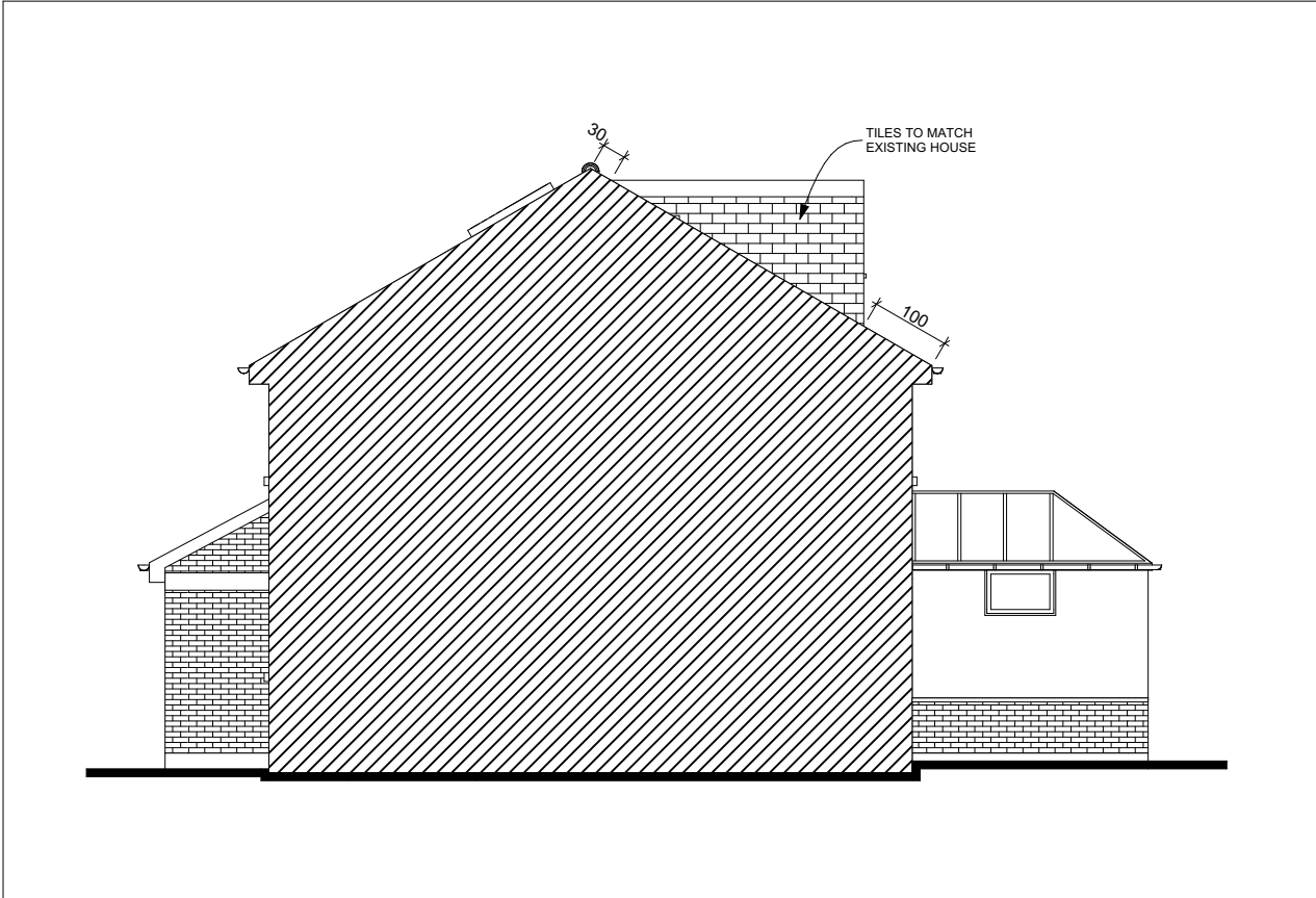
SIDE (NORTH WEST) ELEVATION PROPOSED 1:100
