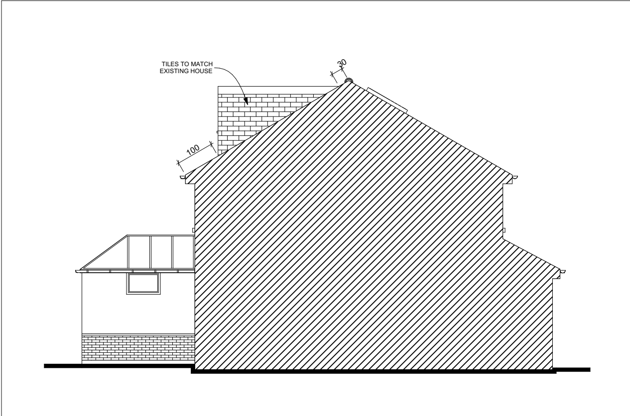
SIDE (SOUTH EAST) ELEVATION PROPOSED 1:100
