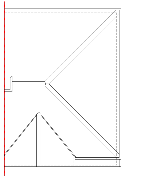
3 Existing Roof Plan 1:100
