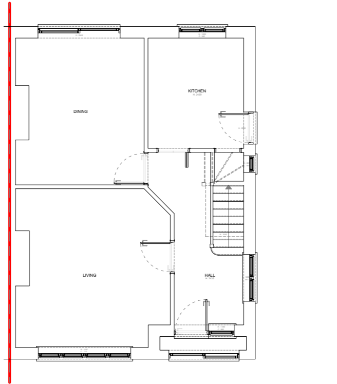
1 Existing Ground Floor Plan 1:100
