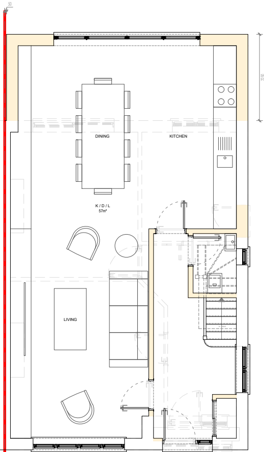
1 Proposed Ground Floor Plan 1:100
