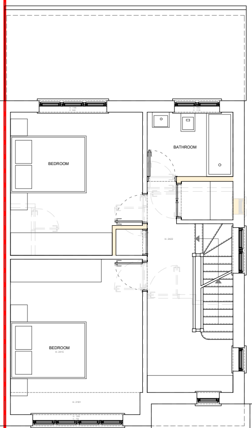
2 Proposed First Floor Plan 1:100
