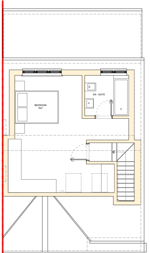
3 Proposed Loft Floor Plan 1:100
