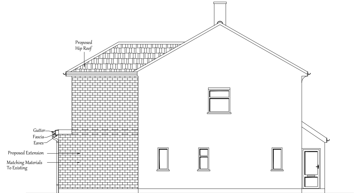
PROPOSED FLANK SIDE ELEVATION
