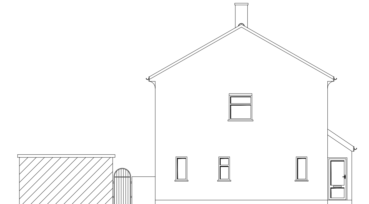
EXISTING FLANK SIDE ELEVATION
