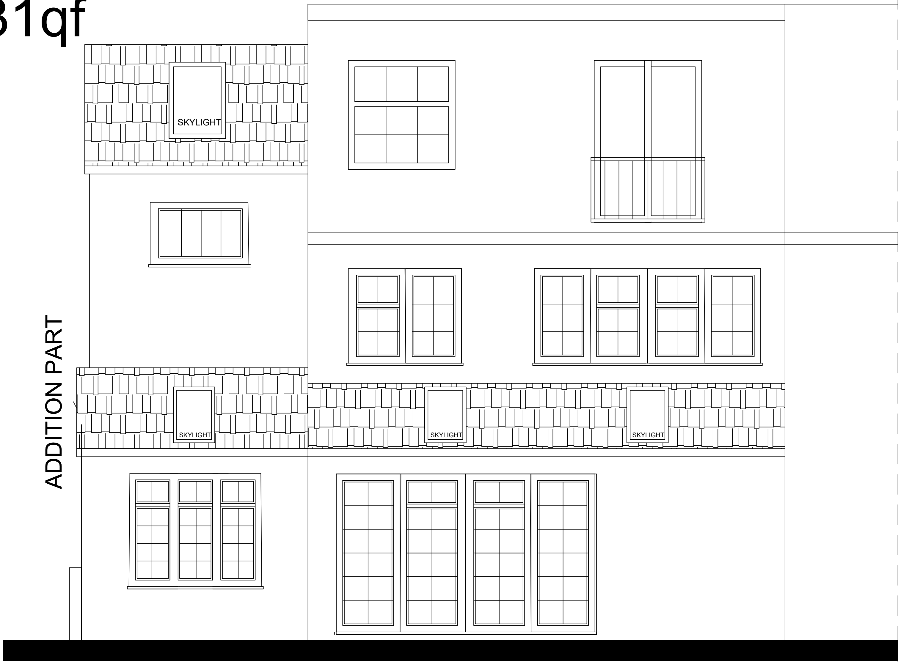
PROPOSED REAR VIEW ELEVATION
