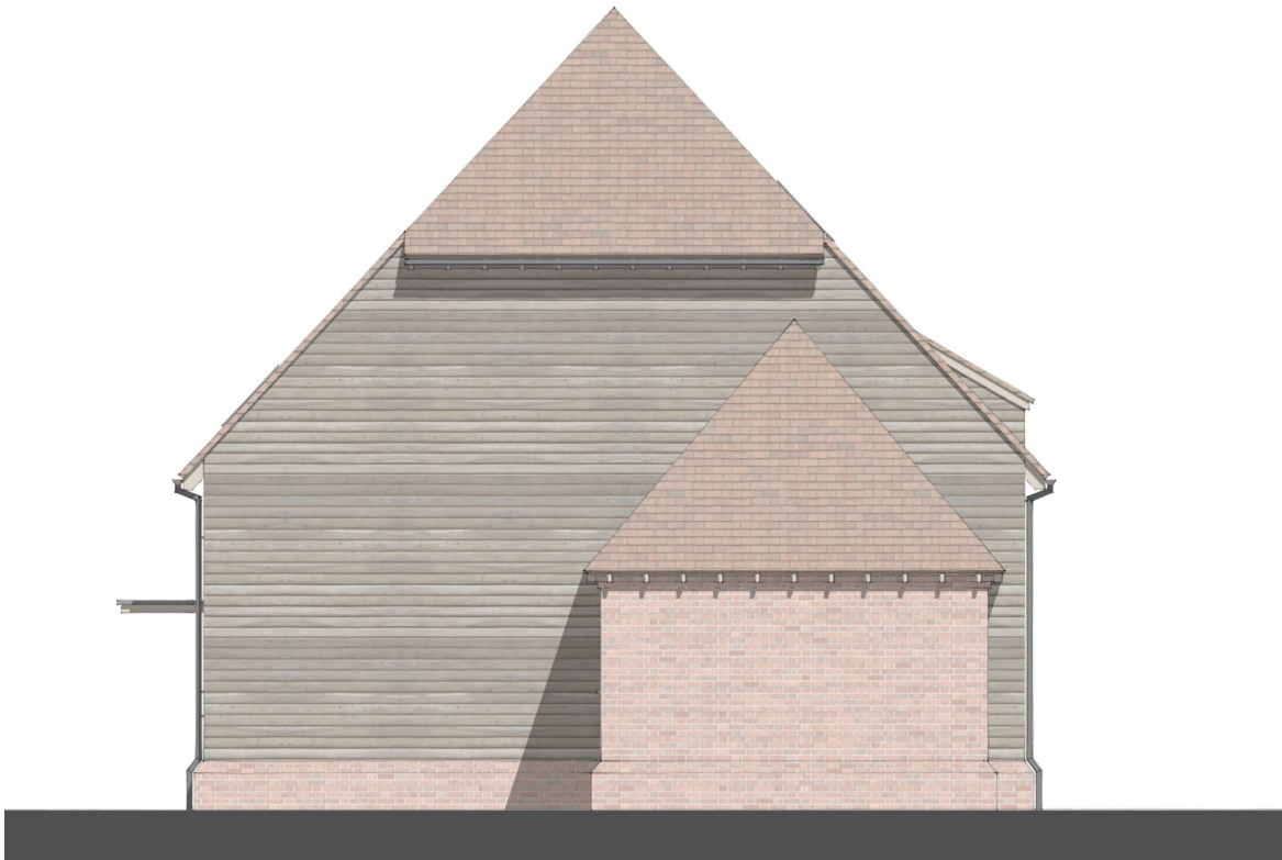
02 PLOT 2 WEST ELEVATION 1:100
