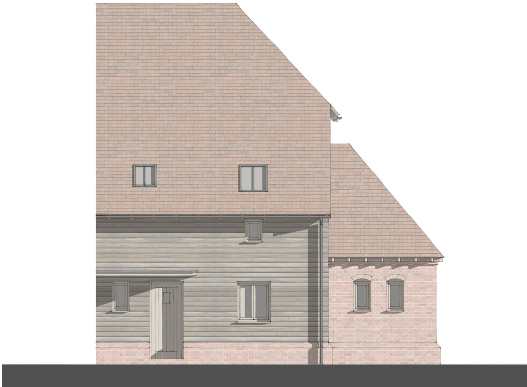
01 PLOT 2 NORTH ELEVATION 1:100
