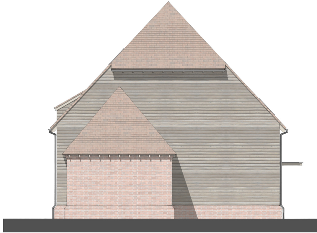
02 PLOT 15 EAST ELEVATION 1:100
